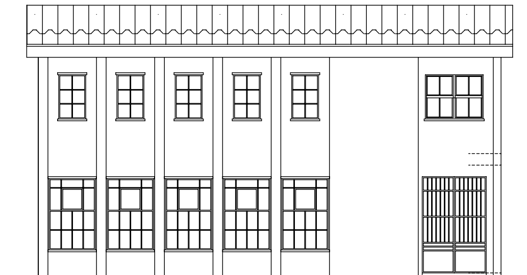
ALZADO PRINCIPAL
