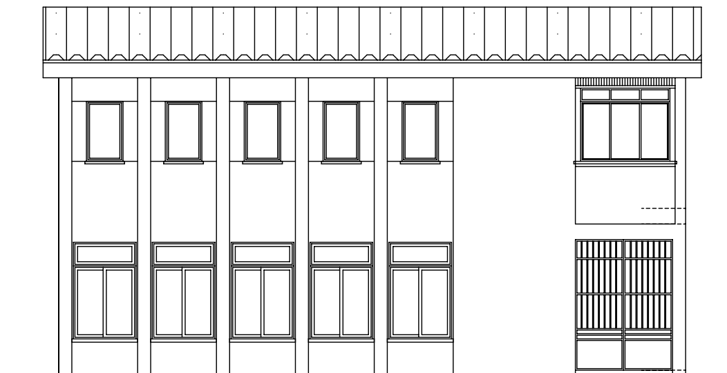
ALZADO PRINCIPAL
