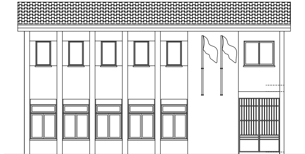
ALZADO PRINCIPAL
